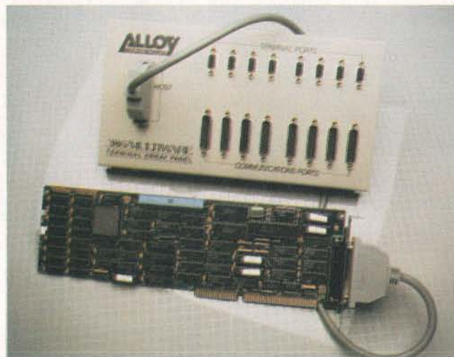
Alloy's IMP8 board supports eight users through the RS-232C panel.
